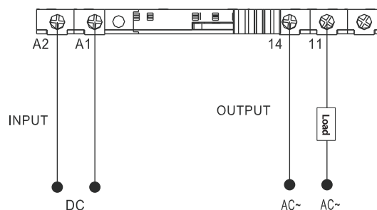
WITH SOCKET SNC05-E-A
