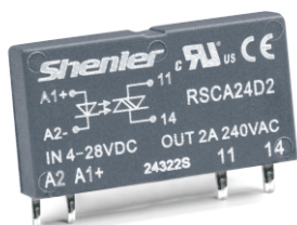
Relay
