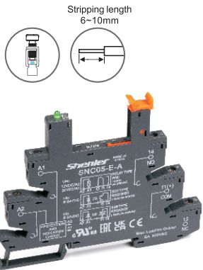
SNC05-E-A
