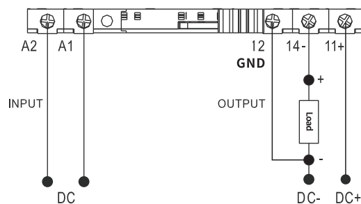
WITH SOCKET SNB05-E-A D & SNB05-ST-A D For Inductive Load
