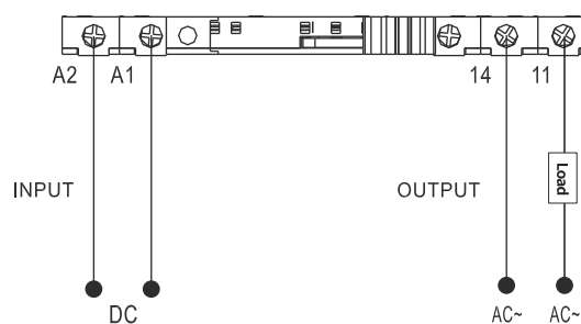
WITH SOCKET SNB05-E-A&SNB05-ST-A
