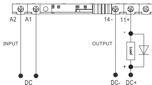
WITH SOCKET SNC05-E-A For Resistive Load
